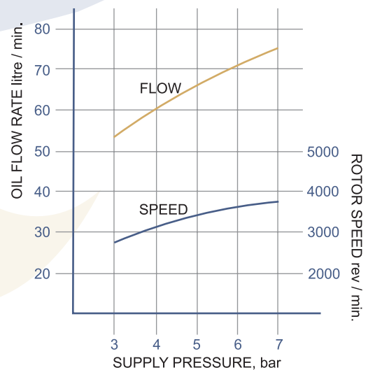
PERFORMANCE CURVES Typical rotor performance for SAE 30 OIL @ 75°C
